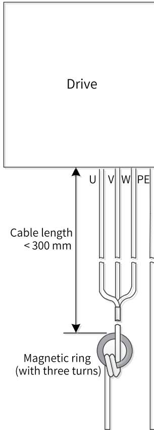
Figure 5-2 Installation of the magnetic ring
