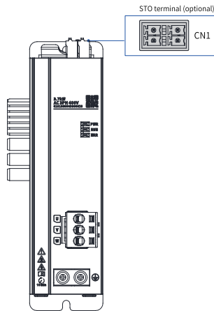
Figure 3-6 STO terminal arrangement of the drive unit (single-axis)
